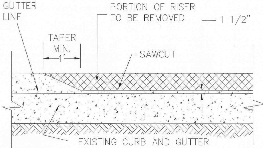
SAWCUT CURB REMOVAL PROFILE
