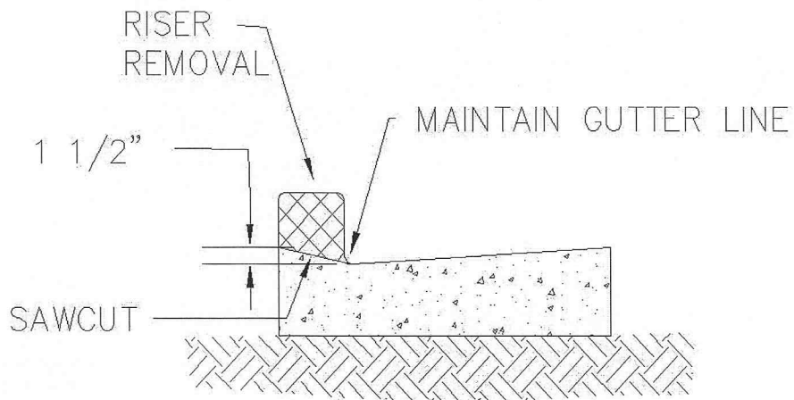
SAWCUT CURB REMOVAL CROSS SECTION
